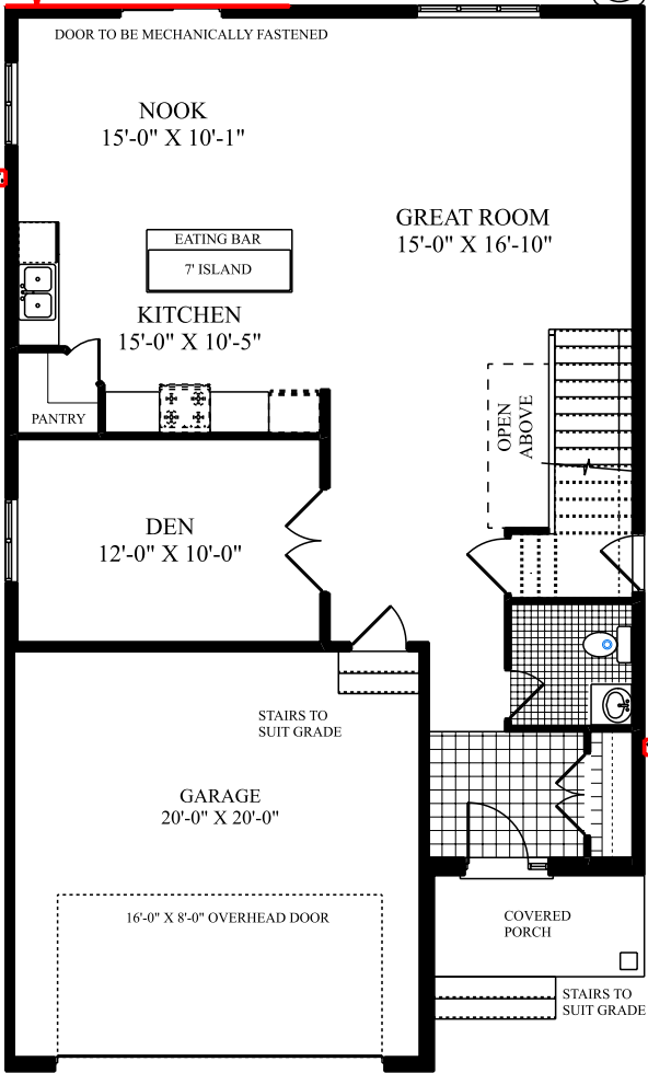
THE ROBIN IV ELEVATION A - 2540 SQ. FT. ELEVATION B - 2545 SQ. FT.
